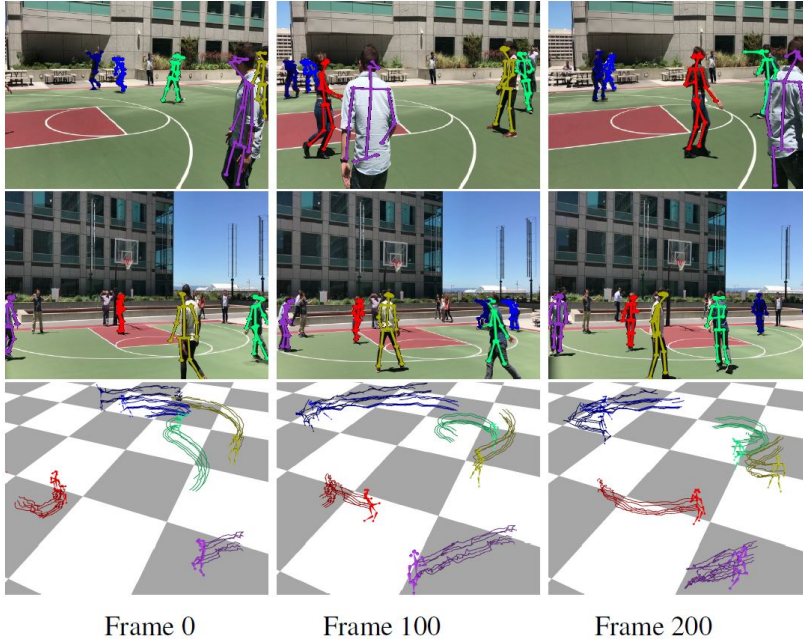
Figure 13: We illustrate the output of Tesseract on the Tagging sequence. The top two row portray the projections of keypoints on two views, while the bottom row shows the 3D pose tracking. Observe smooth tracking of people in the wild with moving cameras for long duration of time.
