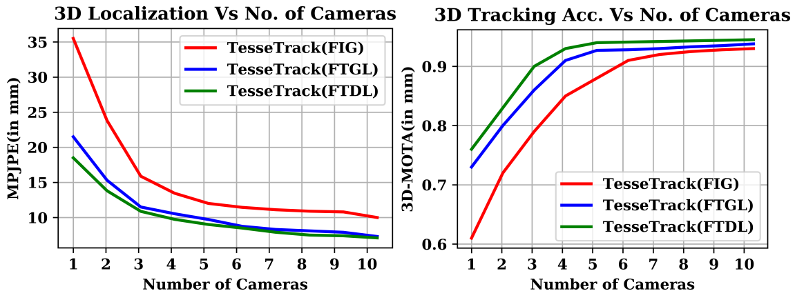
Figure 10: Impact of number of cameras on body joint localization error (MPJPE) (left) and pose tracking accuracy (3D MOTA) (right). Tesseltrack (FTDL) shows the greatest advantage with lower number of cameras.
