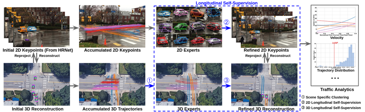
Figure 2: Framework for self-supervised 4D reconstruction of repetitious activity. Our method takes off-the-shelf 2D keypoint detections as input, reconstructs 3D keypoints with an active shape model, fits an analytic trajectory model to each vehicle’s 3D poses along with frames, and accumulates them over time. Then, for 2D self-supervision, good keypoints from initial detections are selected as “2D experts” to refine bad 2D keypoints. For 3D, the accumulated 3D trajectories are clustered and the mean trajectories are used as “3D experts” to refine 3D poses. The reconstruction could be applied to traffic analysis such as velocity estimation and anomaly analysis.
